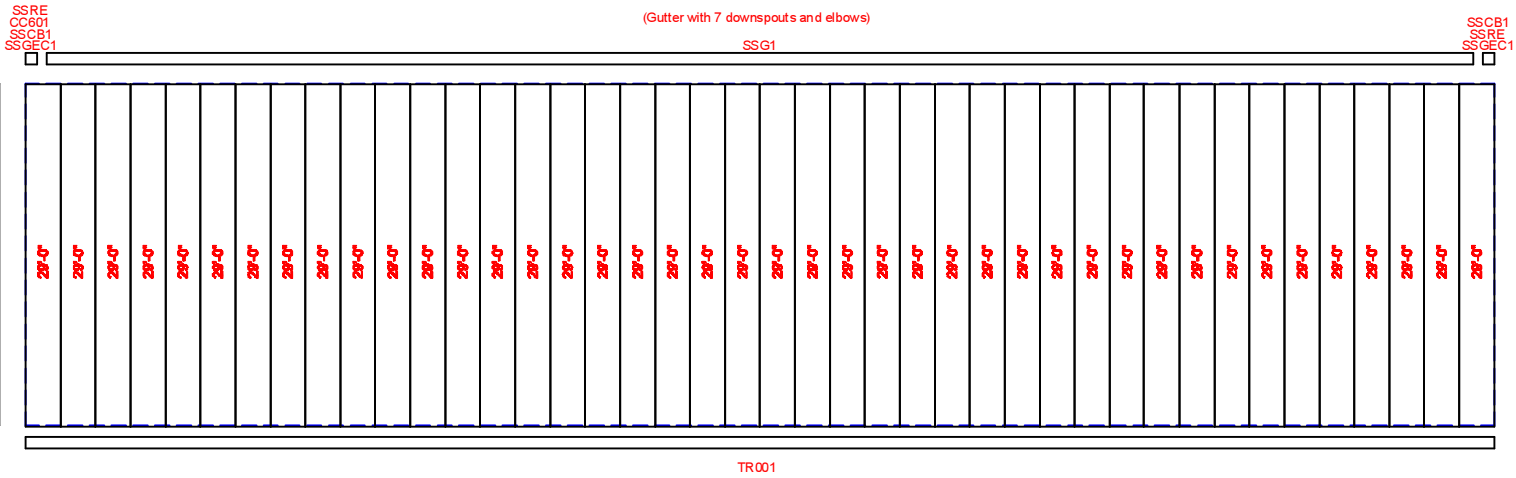
SIDEWALL SHEETING & TRIM: FRAME LINE A PANELS: 26 Ga. CGR - NEED COLOR
