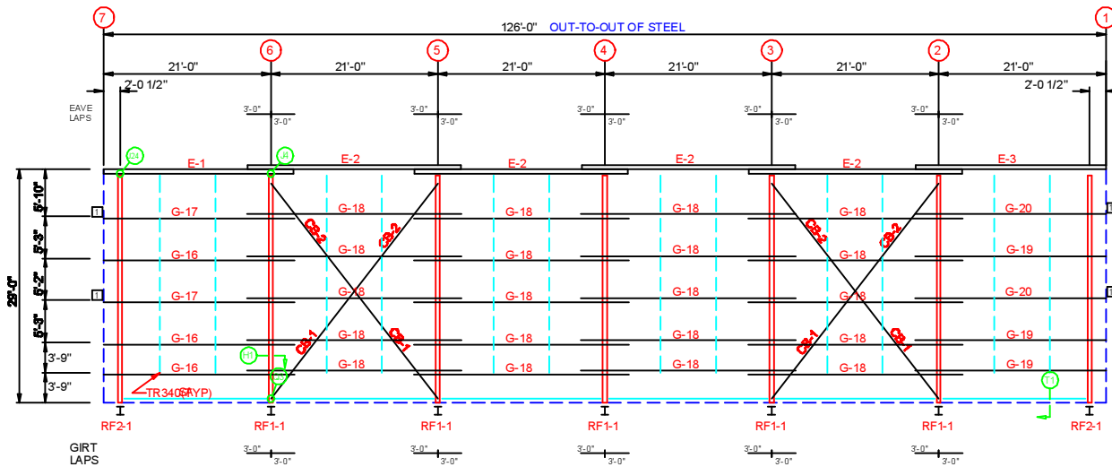
SIDEWALL FRAMING: FRAME LINE H
