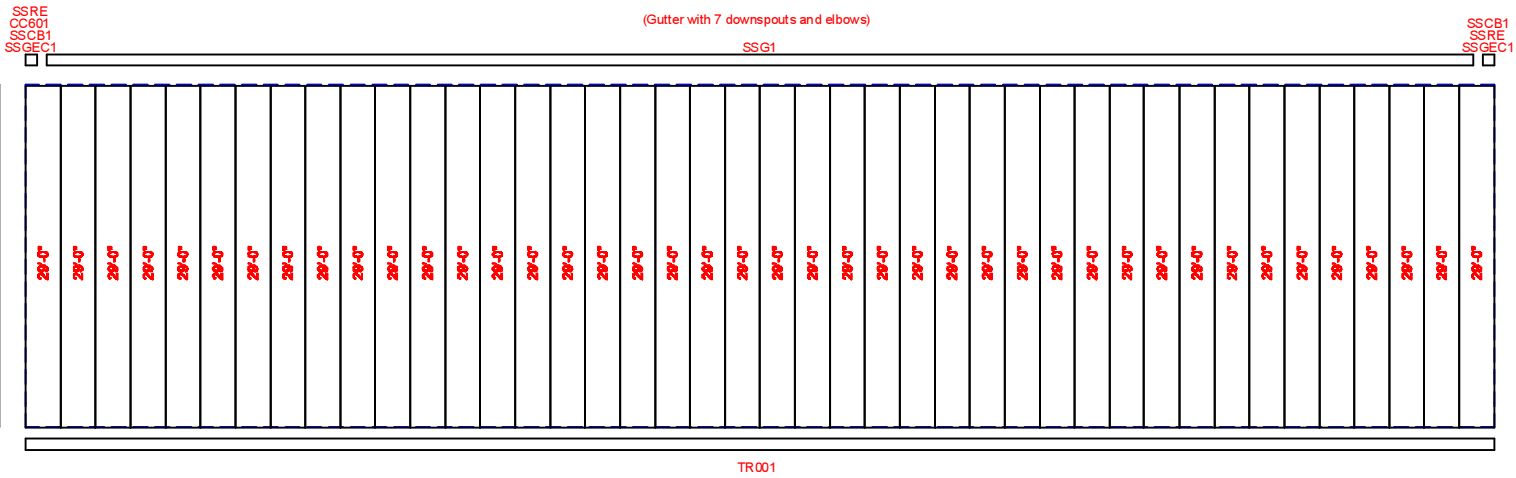
SIDEWALL SHEETING & TRIM: FRAME LINE H PANELS: 26 Ga. CGR - NEED COLOR
