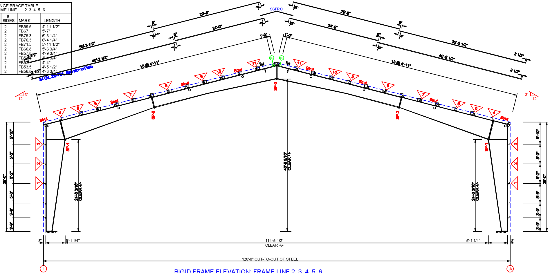
RIGID FRAME ELEVATION: FRAME LINE 2 3 4 5 6
